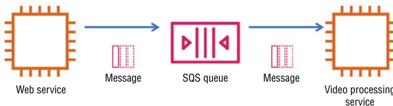
FIGURE 10.3 SQS workflow
