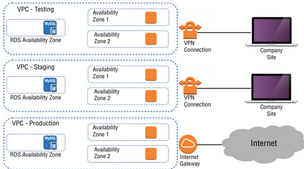
FIGURE 2.1 A multi-VPC infrastructure for a development environment
