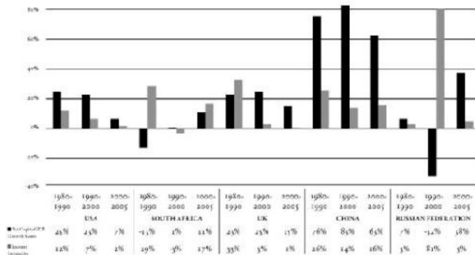
Figure 1. Per Capita PPP GDP Growth Rates vs. Income Inequality Growth Rates for Selected Countries, 1980–2005
